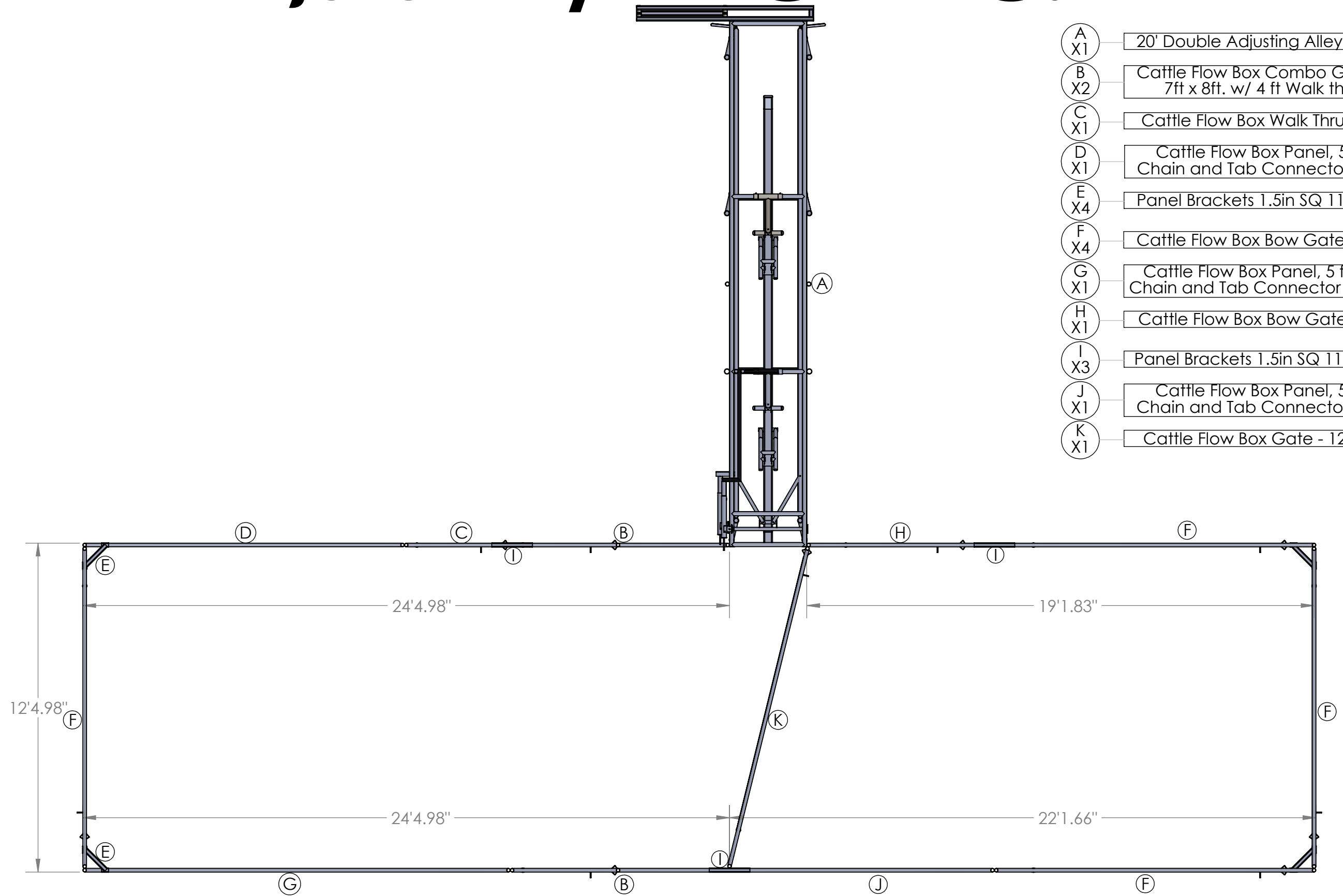
DSU Special Cattle Flow Box
