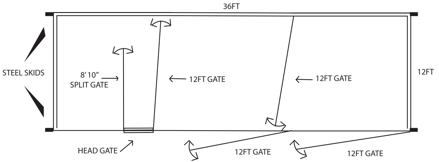
12FT X 36FT CALVING SHED (SAME CONFIGURATION MAY BE USED IN OUR 12FT X 24FT)
